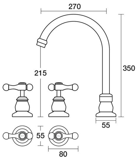
Tudor Sink Set XL Hob Swivel Lever Ceramic Disc B31.053.3.06 - Chrome / Sienna Red
