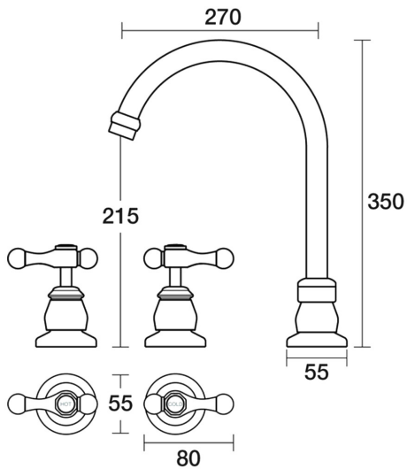
Tudor Sink Set XL Hob Swivel Lever Ceramic Disc B31.053.3.24 - Brushed Gunmetal
