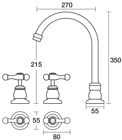
Tudor Sink Set XL Hob Swivel Lever Ceramic Disc B31.053.3.45 - Native Brass
