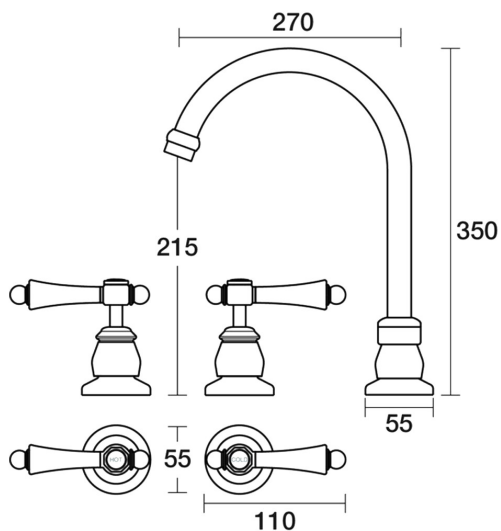
Tudor Sink Set XL Hob Swivel Porcelain Lever Ceramic Disc B31.053.4.04 - Chrome / Ivory
