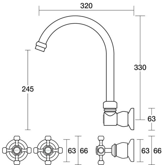
Tudor Sink Set XL Wall Swivel B31.054.1.13 - Gold / White
