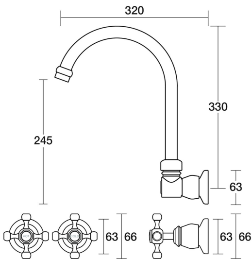
Tudor Sink Set XL Wall Swivel Ceramic Disc B31.054.2.19 - 23k Brushed Brass Gold
