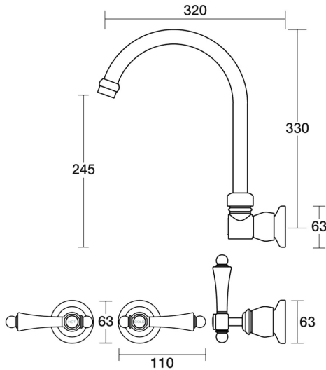
Tudor Sink Set XL Wall Swivel Porcelain Lever Ceramic Disc B31.054.4.12 - 23k Brushed Gold
