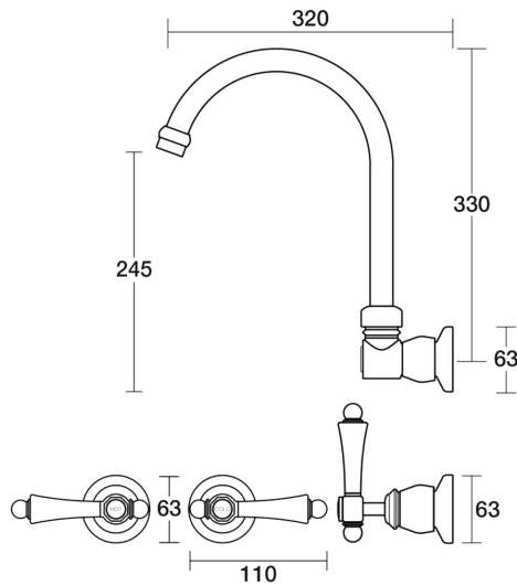
Tudor Sink Set XL Wall Swivel Porcelain Lever Ceramic Disc B31.054.4.23 - Gunmetal
