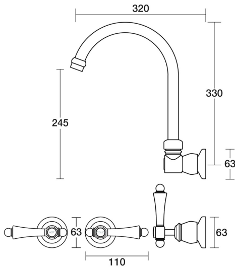
Tudor Sink Set XL Wall Swivel Porcelain Lever Ceramic Disc B31.054.4.52 - Burnished
