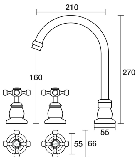
Tudor Spa Set Hob Swivel B31.061.1.13 - Gold / White
