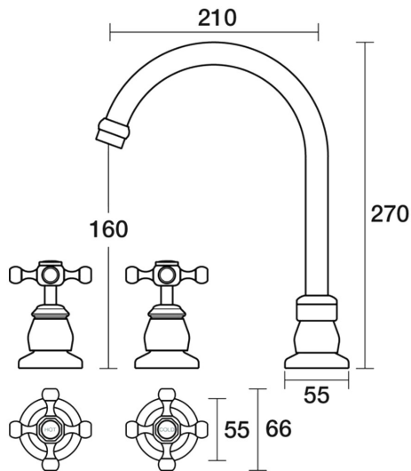
Tudor Spa Set Hob Swivel B31.061.1.24 - Brushed Gunmetal
