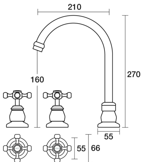
Tudor Spa Set Hob Swivel Ceramic Disc B31.061.2.26 - Black Sapphire
