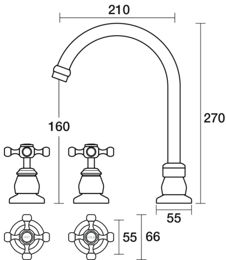
Tudor Spa Set Hob Swivel Ceramic Disc B31.061.2.40 - Rumbled Brass
