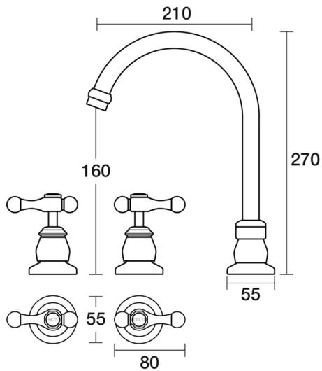
Tudor Spa Set Hob Swivel Lever Ceramic Disc B31.061.3.02 - Brushed Chrome
