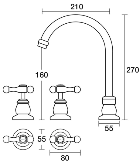
Tudor Spa Set Hob Swivel Lever Ceramic Disc B31.061.3.16 - Gold / Sienna Red
