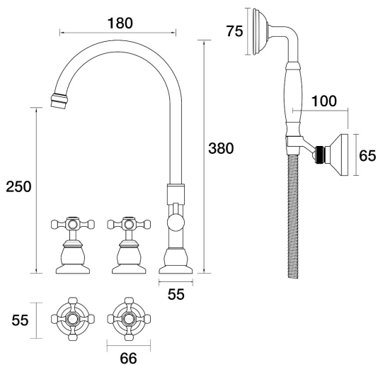
Tudor Spa Set Hob Swivel Divertor Set with Handshower & Bracket Ceramic Disc B31.061.5.07 - Chrome / Victorian Green
