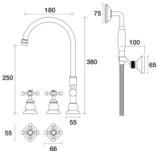
Tudor Spa Set Hob Swivel Divertor Set with Handshower & Bracket Ceramic Disc B31.061.5.15 - Gold / Apricot
