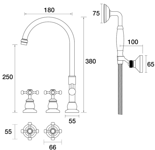
Tudor Spa Set Hob Swivel Divertor Set with Handshower & Bracket Ceramic Disc B31.061.5.25 - Brushed Nickel
