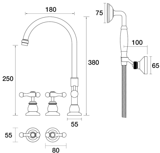
Tudor Spa Set Hob Swivel Divertor Set with Handshower & Bracket Lever Ceramic Disc B31.061.6.34 - Matt Black
