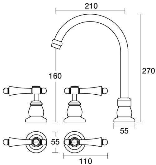
Tudor Spa Set Hob Swivel Porcelain Lever Ceramic Disc B31.061.7.01 - Chrome
