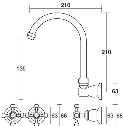
Tudor Spa Set Wall Swivel B31.062.1.03 - Chrome / White
