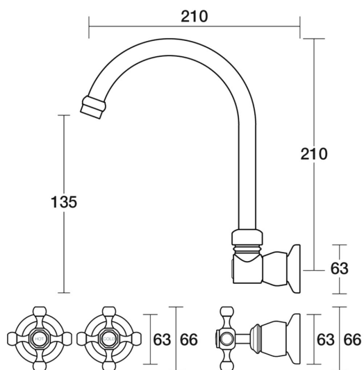
Tudor Spa Set Wall Swivel
