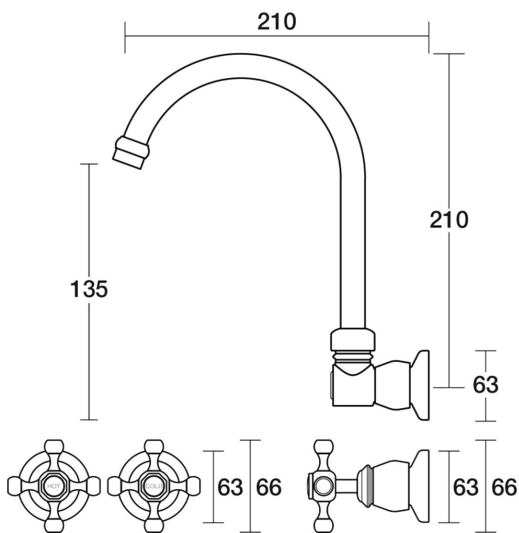
Tudor Spa Set Wall Swivel B31.062.1.27 - Satin Pearl
