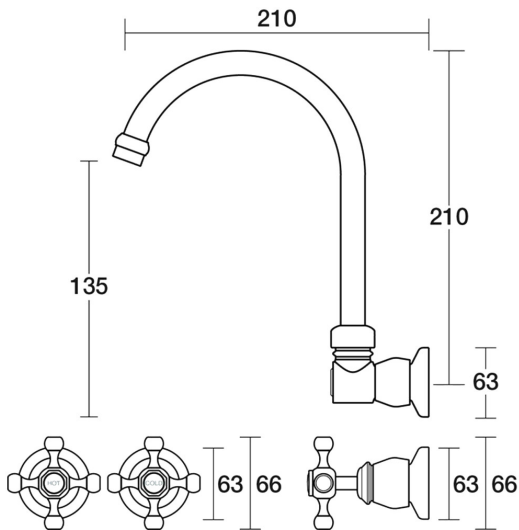
Tudor Spa Set Wall Swivel B31.062.1.43 - Brass
