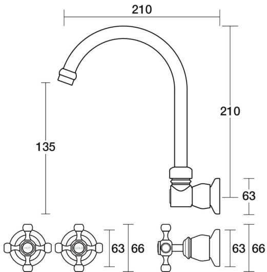
Tudor Spa Set Wall Swivel B31.062.1.45 - Native Brass
