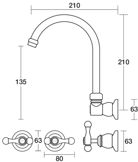
Tudor Spa Set Wall Swivel Lever Ceramic Disc B31.062.3.07 - Chrome / Victorian Green
