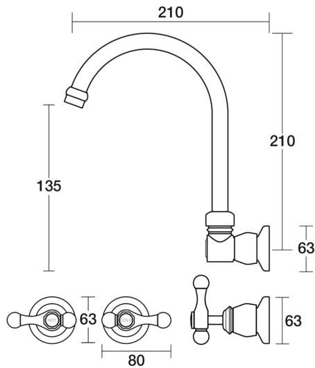
Tudor Spa Set Wall Swivel Lever Ceramic Disc B31.062.3.26 - Black Sapphire
