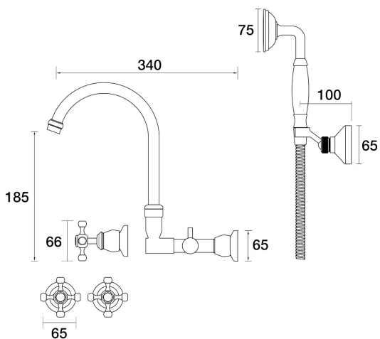
Tudor Spa Set Wall Swivel Divertor Set with Handshower & Bracket B31.062.4.52 - Burnished
