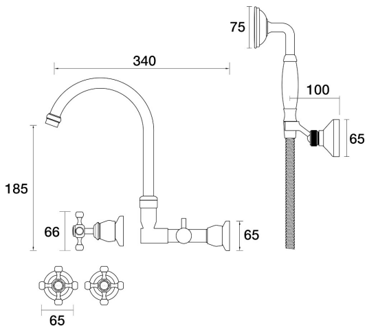
Tudor Spa Set Wall Swivel Divertor Set with Handshower & Bracket Ceramic Disc B31.062.5.06 - Chrome / Sienna Red
