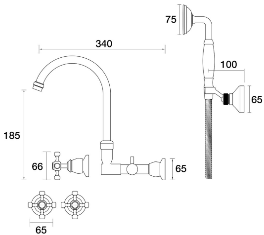
Tudor Spa Set Wall Swivel Divertor Set with Handshower & Bracket Ceramic Disc B31.062.5.52 - Burnished
