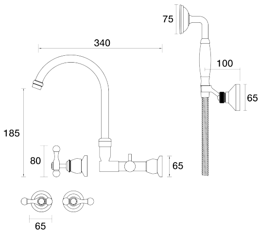
Tudor Spa Set Wall Swivel Divertor Set with Handshower & Bracket Lever Ceramic Disc B31.062.6.01 - Chrome
