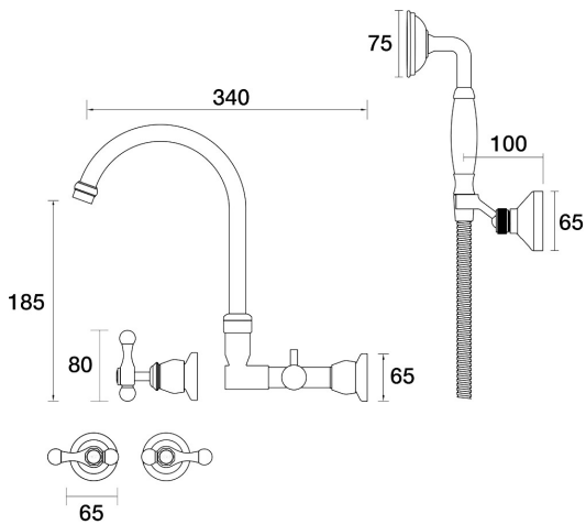
Tudor Spa Set Wall Swivel Divertor Set with Handshower & Bracket Lever Ceramic Disc B31.062.6.04 - Chrome / Ivory
