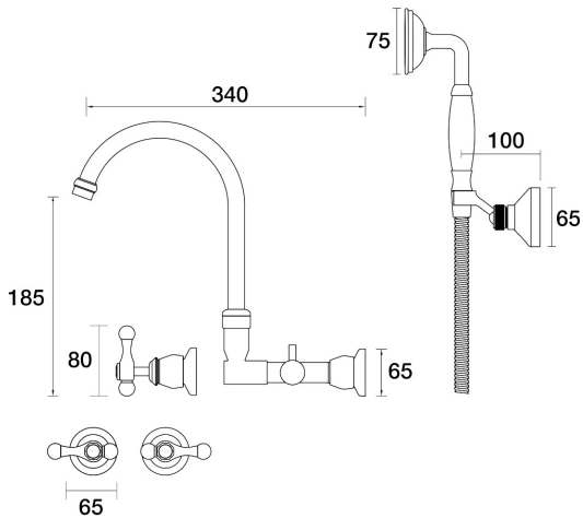
Tudor Spa Set Wall Swivel Divertor Set with Handshower & Bracket Lever Ceramic Disc B31.062.6.17 - Gold / Victorian Green
