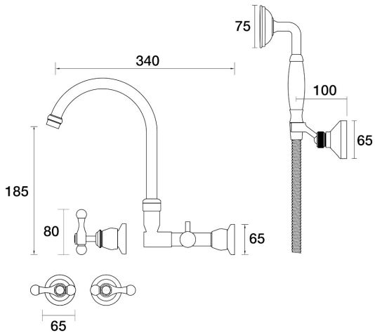
Tudor Spa Set Wall Swivel Divertor Set with Handshower & Bracket Lever Ceramic Disc B31.062.6.21 - Brushed Rose Gold
