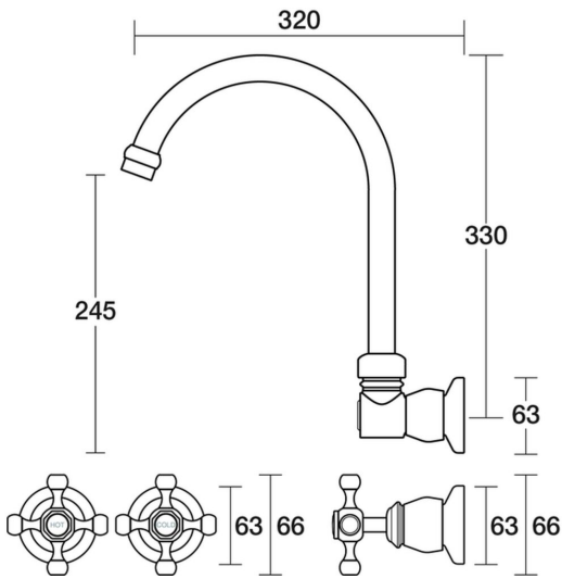
Tudor Spa Set XL Wall Swivel B31.064.1.01 - Chrome
