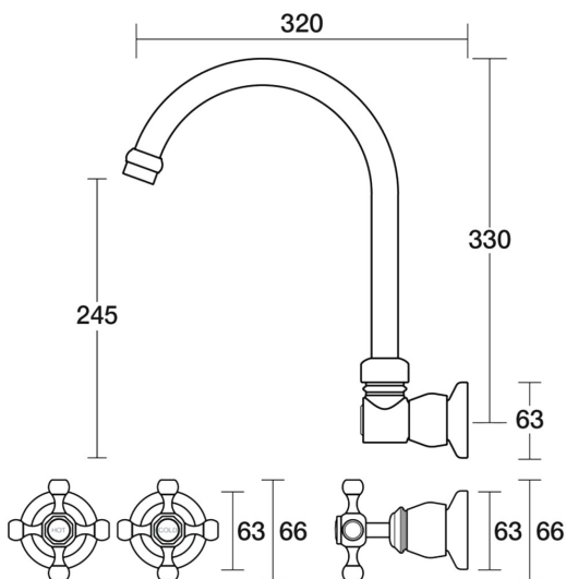
Tudor Spa Set XL Wall Swivel Ceramic Disc B31.064.2.32 - Midnight Black
