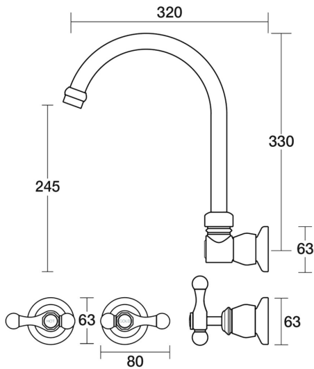
Tudor Spa Set XL Wall Swivel Lever Ceramic Disc B31.064.3.11 - 23k Gold
