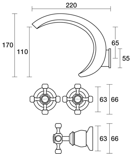
Tudor Spa Set Wall Deluxe B31.066.1.39 - Antique Bronze
