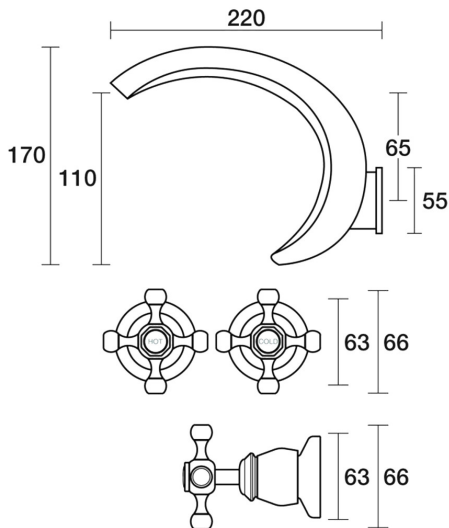
Tudor Spa Set Wall Deluxe Ceramic Disc B31.066.2.25 - Brushed Nickel
