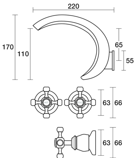
Tudor Spa Set Wall Deluxe Ceramic Disc B31.066.2.57 - Matt Nickel
