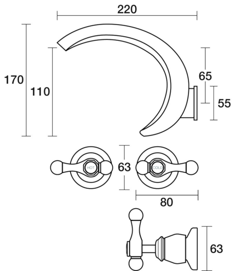
Tudor Spa Set Wall Deluxe Lever Ceramic Disc B31.066.3.43 - Brass
