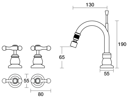
Tudor Bidet Set Fixed Lever Ceramic Disc B31.071.3.23 - Gunmetal
