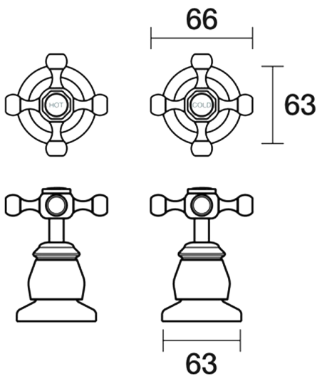
Tudor Top Assemblies Wall Pair B31.082.1.01 - Chrome
