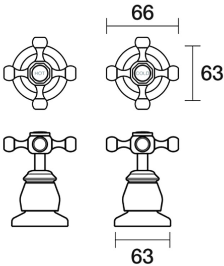
Tudor Top Assemblies Wall Pair Ceramic Disc B31.082.2.17 - Gold / Victorian Green
