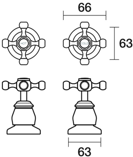
Tudor Top Assemblies Wall Pair Ceramic Disc B31.082.2.23 - Gunmetal
