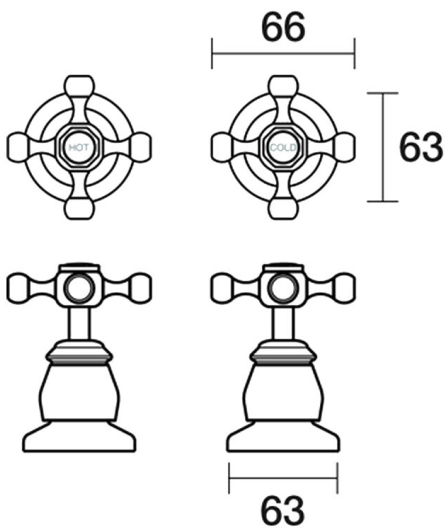
Tudor Top Assemblies Wall Pair Ceramic Disc B31.082.2.39 - Antique Bronze
