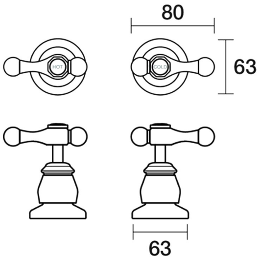
Tudor Top Assemblies Wall Pair Lever Ceramic Dia. 80.3.07 - Chrome / Victorian Green
