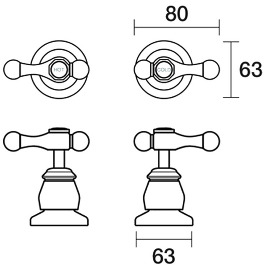
Tudor Top Assemblies Wall Pair Lever Ceramic Part No. 082.3.10 - Chrome / Gold
