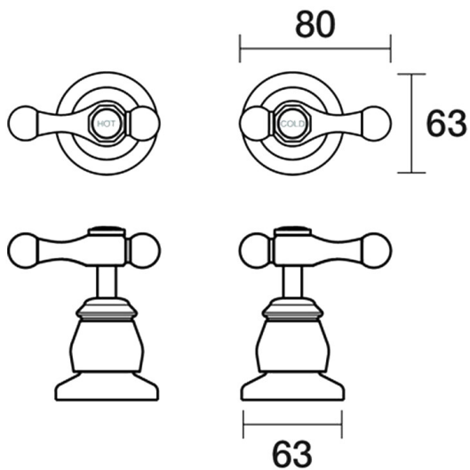
Tudor Top Assemblies Wall Pair Lever Ceramic Dia. 80mm 082.3.13 - Gold / White
