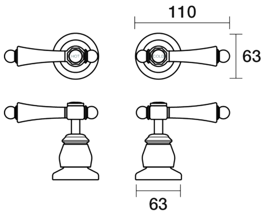
Tudor Top Assemblies Wall Pair Porcelain Lever Ceramic Disc B31.082.4.01 - Chrome
